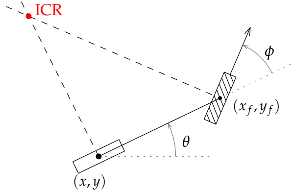
Figure 1.11: The instantaneous center of rotation.
