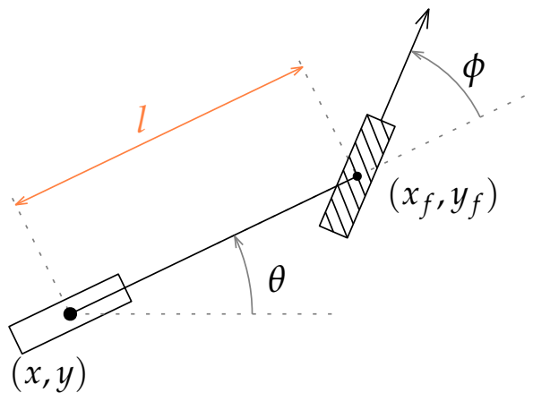
Figure 1.10: The bicycle model.
